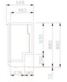
SIDE VIEW < 900mm >
