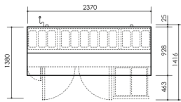
Integral top view
