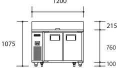
Integral front elevation
